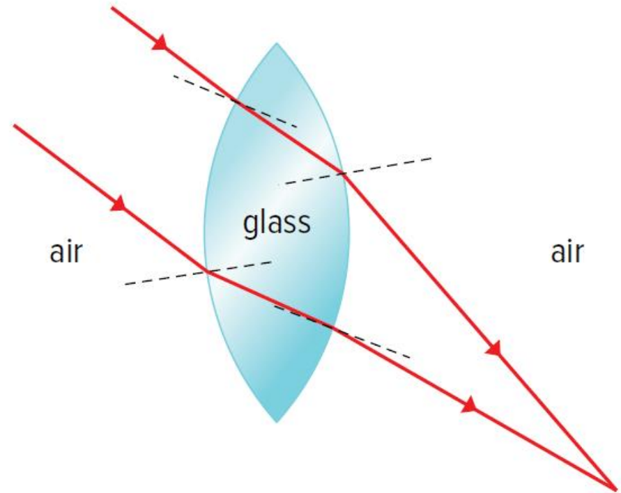
Figure 3.39: Converging lens
